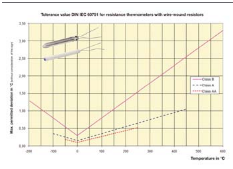
The new DIN EN 60751:2009 standard changes the use of platinum resistance thermometers in industrial applications
